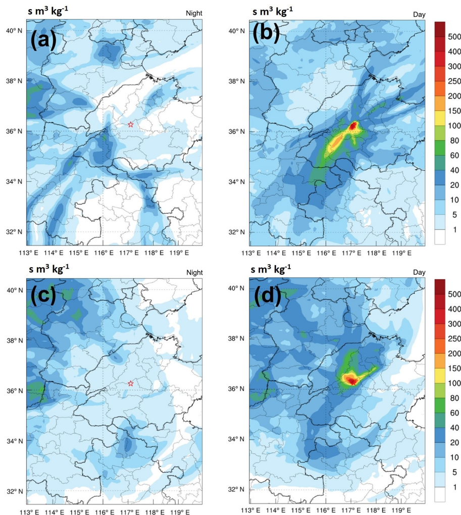
Figure 4. Average distribution of the “footprint” retriplume of the 3 d backward trajectory during (a) spring at nighttime (02:00–08:00 LT), (b) spring in the afternoon (12:00–18:00 LT), (c) winter at nighttime (02:00–08:00 LT), and (d) winter in the afternoon (12:00–18:00 LT). Note that the horizontal resolution is 0.1^\circ .
