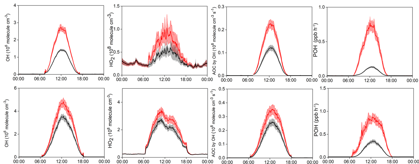
Figure 8. Model-simulated average diurnal variations of OH, HO 2 , AOC, and primary OH production rate (PO H ) at Mt. Tai in winter (upper panel) and spring (lower panel), with (red) and without (black) constraints of HONO measurement data. Note that the model only considers the homogenous HONO formation from OH + NO reactions. Shaded area indicates the standard error.
