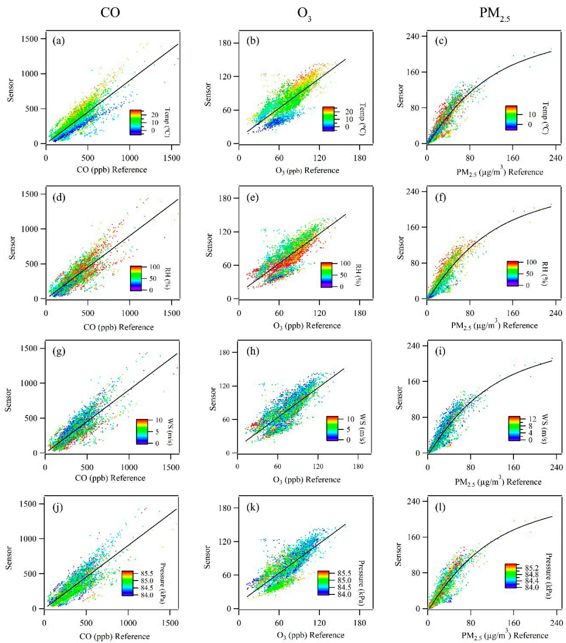
Figure 6. Scatter plots of sensor data and reference data, color-coded with meteorological factors: (a–c) temperature, (d–f) relative humidity, (g–i) wind speed, and (j–l) pressure.
