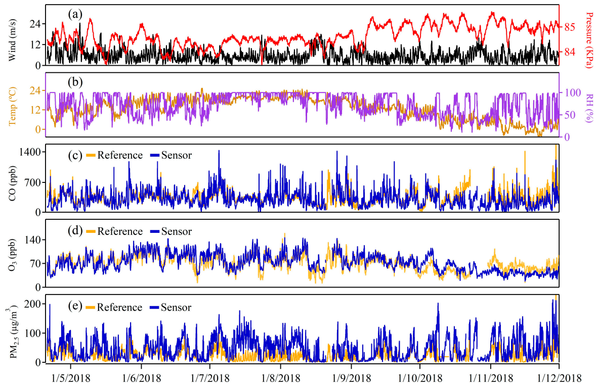
Figure 3. Time series of the measured meteorological and air quality data at Mt. Tai from 20 April to 30 November 2018: (a) Wind speed (WS) and pressure, (b) temperature (T) and relative humidity (RH), (c) CO, (d) O 3 , and (e) PM 2.5 .
