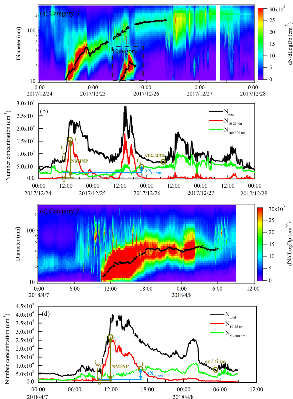
Figure 1. Examples of NPF events in three categories. Black dots in the figures are the fitted D_{pg} . (a) Category 1 on 25 December 2017, in which D_{pg\text{max}} was 24 nm ( < 50 nm), and Category 3 on 24 December 2017, in which D_{pg\text{max}} grew to 163 nm ( > 80 nm); (c) Category 2 on 7 April 2018, in which D_{pg\text{max}} grew to 53 nm (50–80 nm). (b, d) Schematic diagram of t_0 , t_1 , t'_1 , NMINP, and \Delta N_{\text{CCN}100}/\Delta N_{\text{CCN}50} on 24 December 2017 and 7 April 2018 NPF events (a few spikes have been removed from d).
