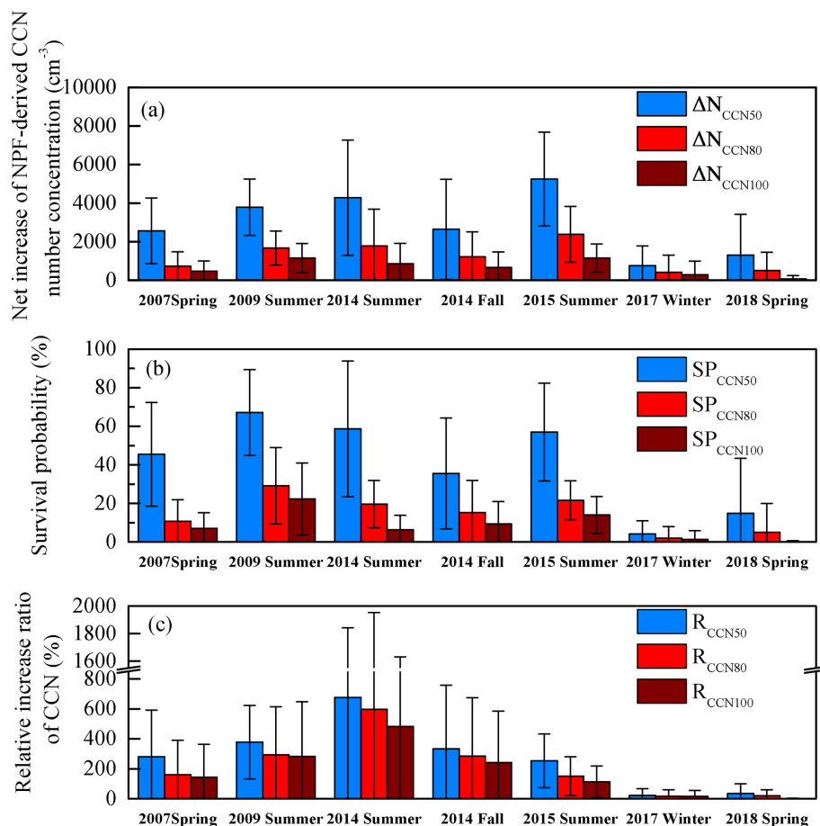
Figure 4. Campaign average of the net increase in the NPF-derived CCN number concentration ( \Delta N_{CCN} , a ), the survival probability of new particles growing to CCN sizes ( SP_{CCN} , b ), and the relative increase ratio of the CCN population ( R_{CCN} , c ) during the seven observation campaigns. The error bars are the standard deviations.
