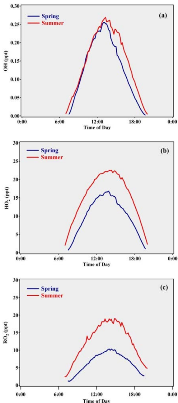
Fig. 7. Model-predicted daytime profiles of (a) OH, (b) HO 2 , and (c) RO 2 at WLQ.
