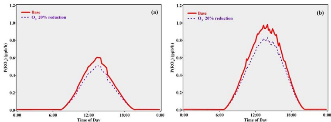
Fig. 8. Sensitivity of RO_x production rates to surface O_3 levels at WLG in (a) spring and (b) summer.
