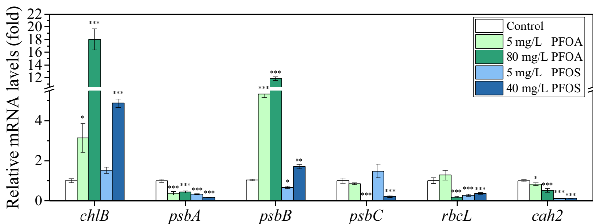
Fig. 5. Relative mRNA levels of 6 genes in the algal cells exposed to 5, 80 mg/L PFOA and 5, 40 mg/L PFOS for 7 days. Statistical significance versus the control group: * p < 0.05 , ** p < 0.01 , *** p < 0.001 .
