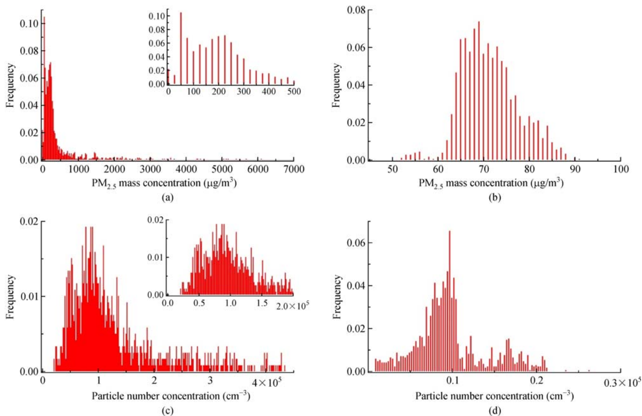
Fig. 2 Distribution of PM_{2.5} mass concentrations at the barbecue restaurants (a) and the SDU site (b), and sub-micron particle number concentration at the barbecue restaurants (c) and the SDU site (d). The insets show the details within a small concentration range
