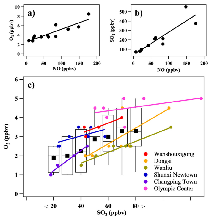
Fig. 4. Scatter plot of (a) O_3 and NO, (b) SO_2 and NO during the Chinese New Year 2007 in Jinan, and (c) O_3 and SO_2 during the Chinese New Year 2016 in Beijing.
