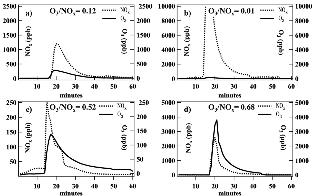
Fig. 2. The concentration of NO x and O 3 as a function of time after lighting the pencil sparkler (a), flash powder (b), cardboard covering flash powder (c) and tobacco (d).
