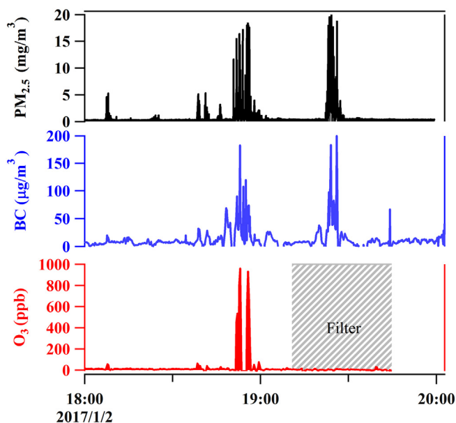
Fig. 3. Unmanned rotorcraft measurement of PM_{2.5} , BC and O_3 in the plumes of display shell emission.
