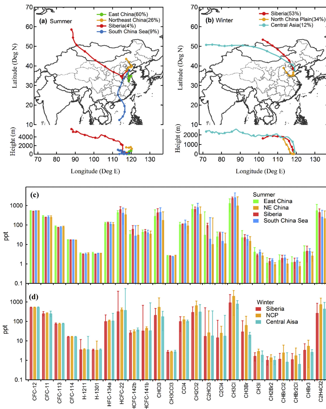
Fig. 6. Five-day HYSPLIT back trajectory clusters and comparison of the associated concentrations of halocarbons in the YelRD region. (a), (c) and (b), (d) stand for summer and winter-spring, respectively. Levels of halocarbons are presented with median \pm SD.
