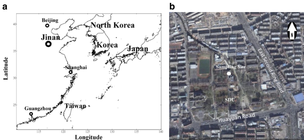
Fig. 1 Location of the atmospheric measurement site. a Location of Jinan. b Sampling site (white dot in the image from Google Earth™)
