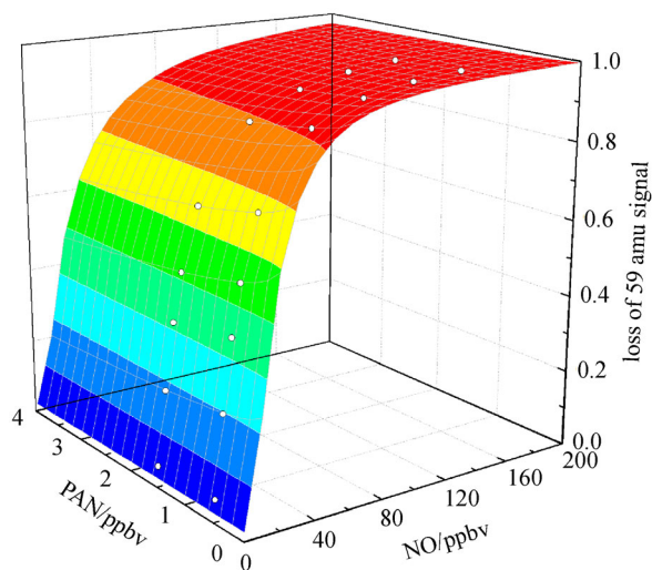
Fig. 4 Effect of NO and PAN concentrations on signal loss at 59 amu
