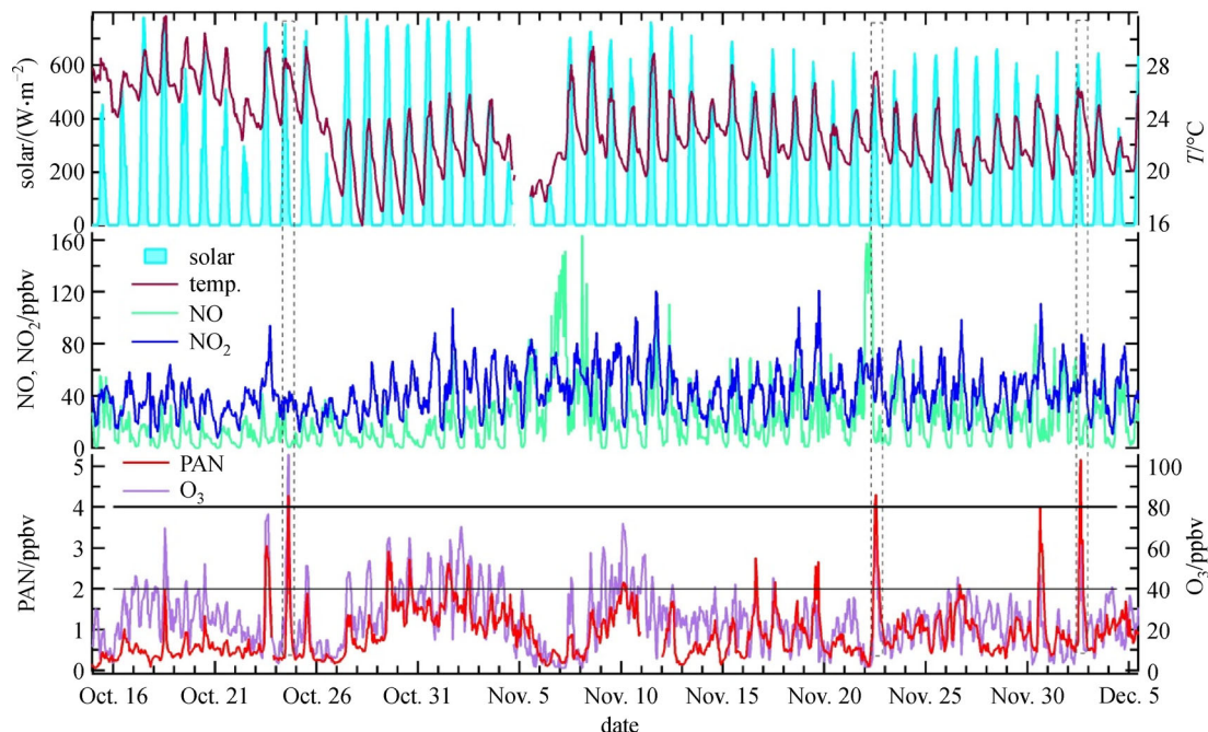
Fig. 6 Time series of concentrations of PAN, O 3 , NO, and NO 2 , and meteorological parameters of solar radiation and temperature for the field measurements
