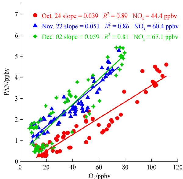
Fig. 8 Scatter plots of PAN versus ozone for three pollution episodes on Oct. 24, Nov. 22, and Dec. 2, 2010. The slope indicates the relative formation efficiency of PAN
